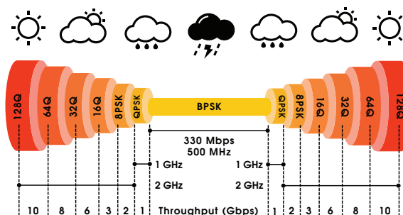
V10g Adaptive Code Modulation and Baud (ACMB)
