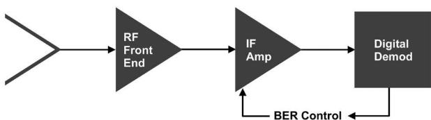
Figure 4. Intelligent AGC with Bit Error Rate Control
