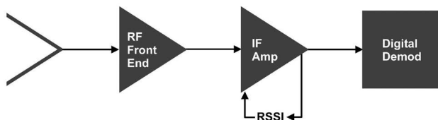
Figure 3. Traditional RSSI Gain Adjustment
