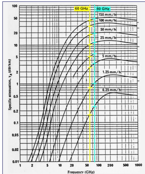
Figure 1. Attenuation due to Rain vs Frequency
