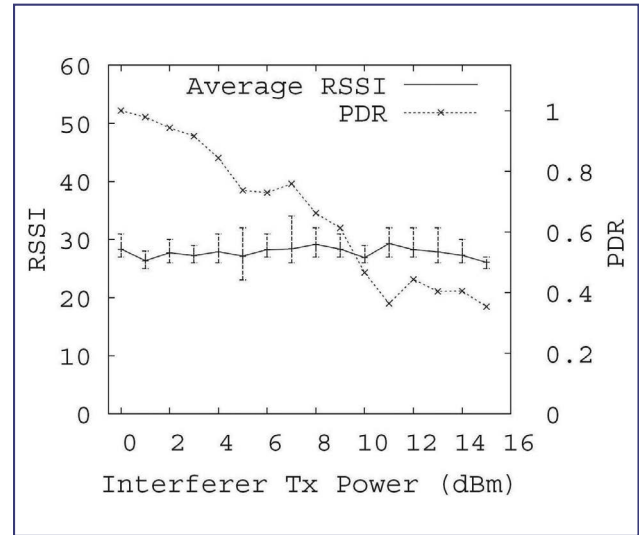
Figure 3. Wireless Link RSSI and PDR with Interference 3
